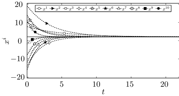
Figure 3: Simulation results using the average consensus algorithm (4.3).
